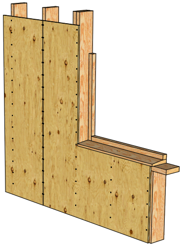
01. Studs, sheathing, blocking
