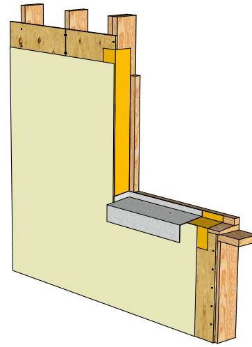
04. Pan flashing
