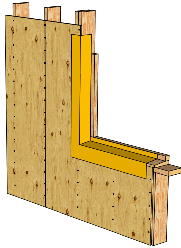
02. Transition membrane
