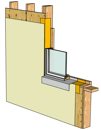
05. Window assembly
