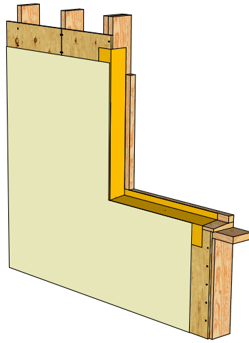
03. Air barrier
