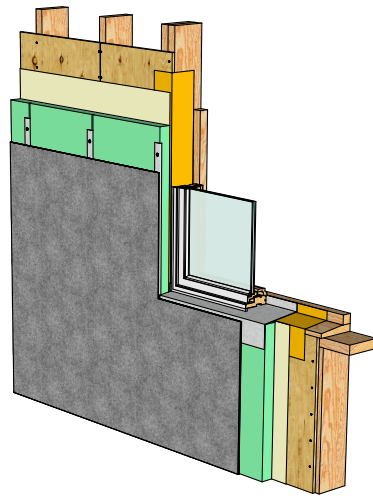
07. Drainage material
