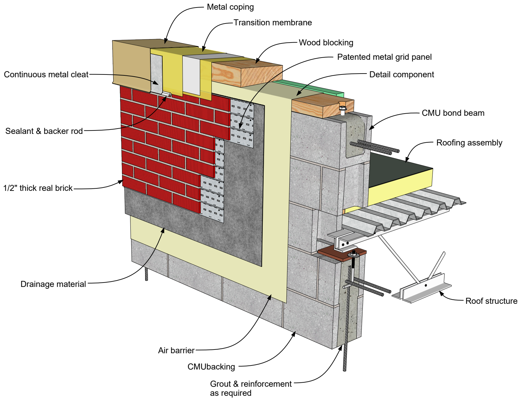
MCS Exterior Wall, CMU Backing | Top of Wall Detail 03.01.06 Rev. 01/26/19
