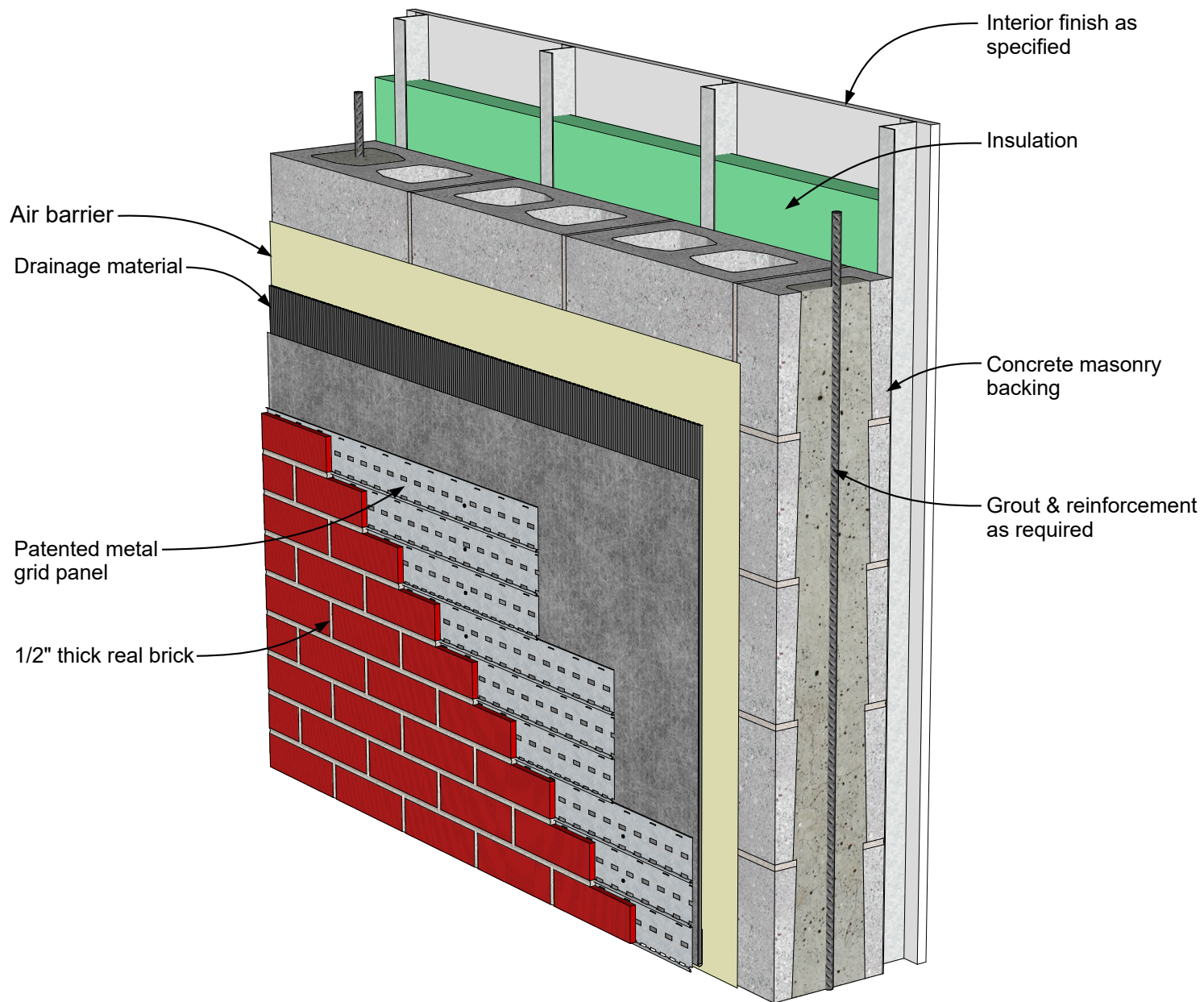
MCS Exterior Wall, CMU Backing Detail 03.01.00 Rev. 01/12/19
